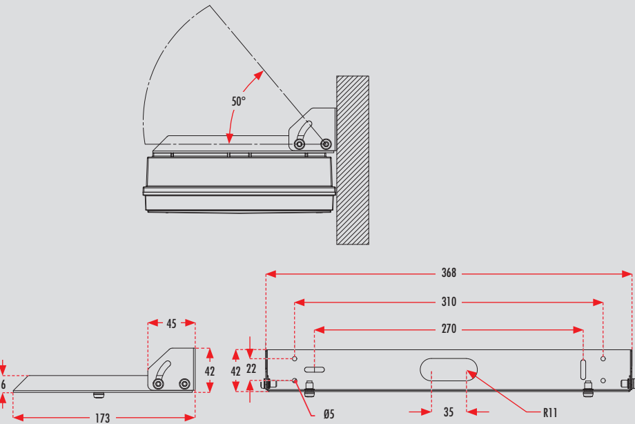
TWT3002 | Wall bracket
