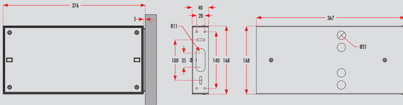
TWT3003 | Flag bracket
