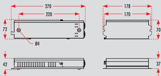
TWSxx92Wx | Electronics unit
