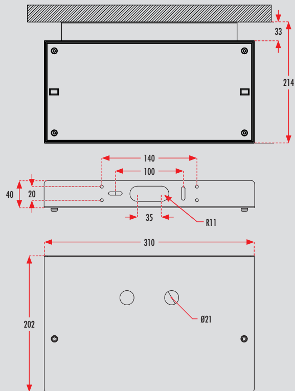
TWT3004 | Ceiling bracket
